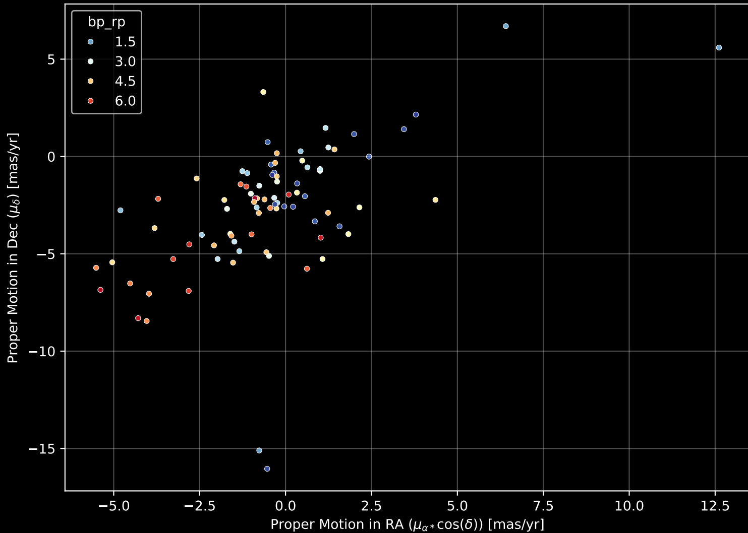
APOGEE DR17 Field: [016+00] Proper Motion Diagram (n= 84)
