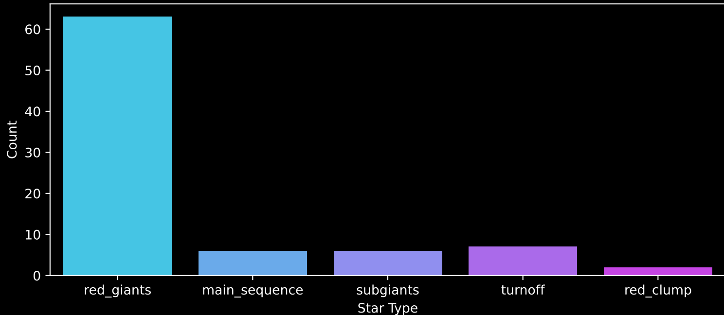
APOGEE DR17 Field: [016+00] Count plot of Star Type
