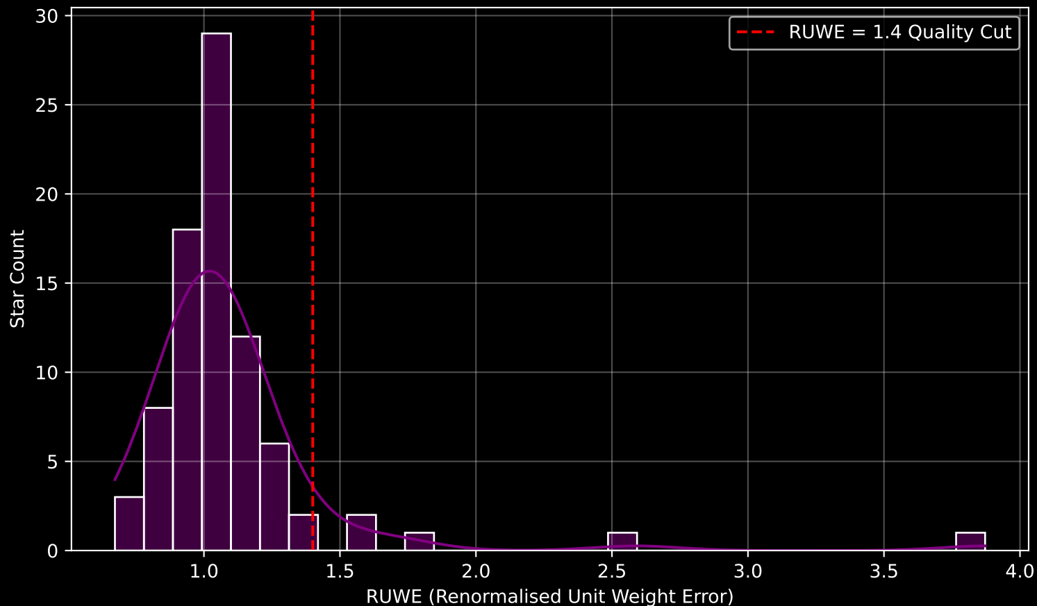
GAPOGEE DR17 Field [016+00] RUWE Distribution (n= 83)
