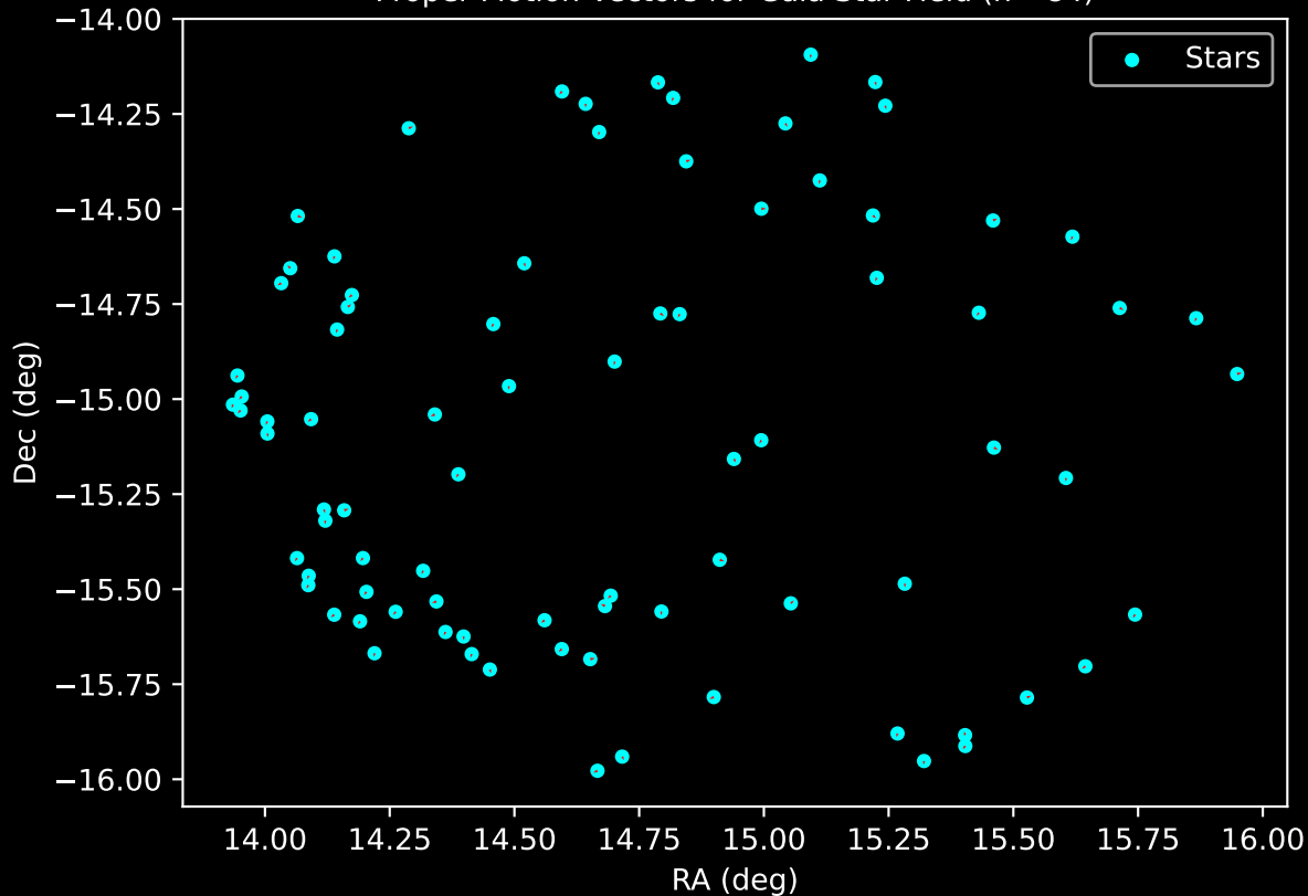
APOGEE DR17 Field: [016+00] Proper Motion Vectors for Gaia Star Field (n= 84)
