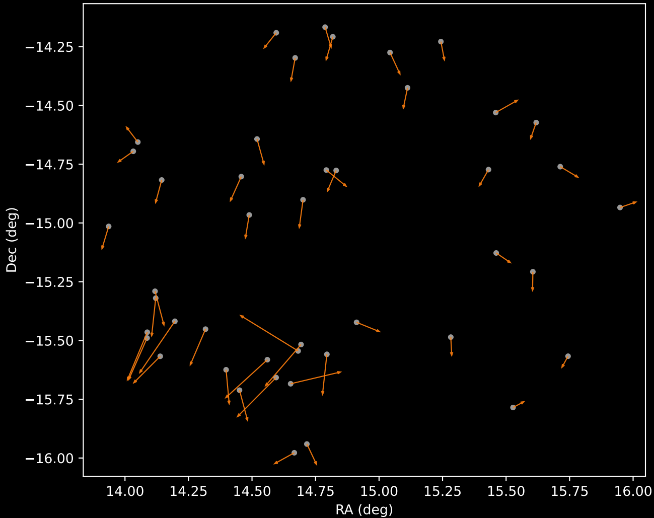
APOGEE DR17 Cluster 2 Proper Motion Vectors (n=45)
