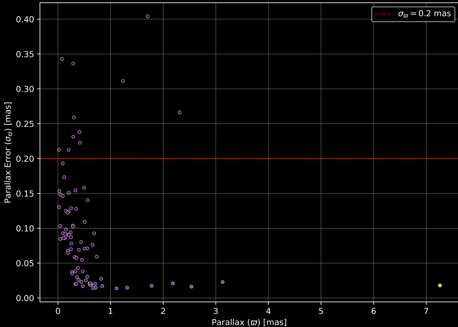
APOGEE DR17 Field: [016+00] Parallax Quality (n= 84)
