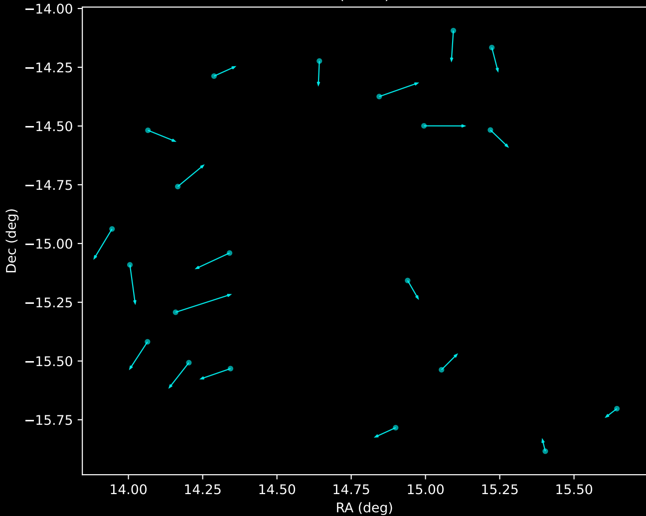
APOGEE DR17 Noise Stream Proper Motion Vectors (n=21)
