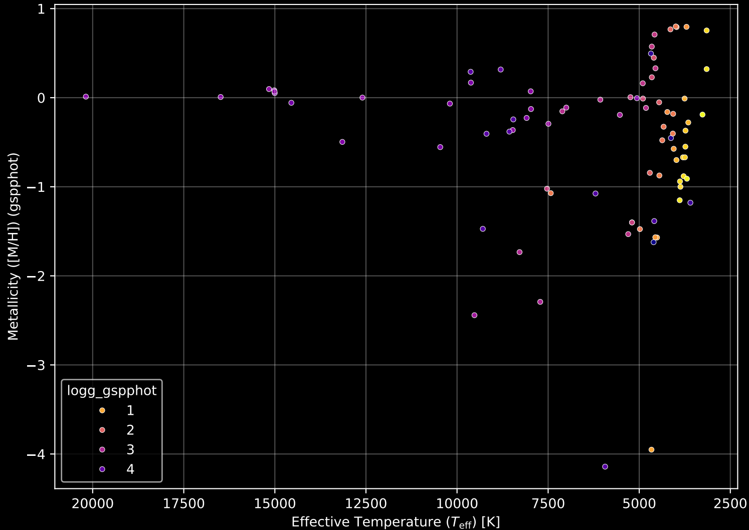
APOGEE DR17 Field: [016+00] Stellar Population Parameters (n= 84)
